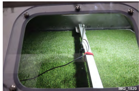
10. Closer view of turf in the chamber before start of testing. (Note no vacuum applied.)
