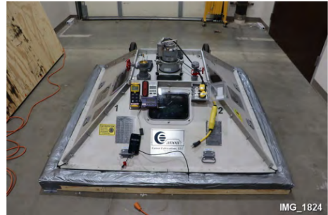
9. Uplift dome placed over turf. (Note duct tape utilized to seal.)
